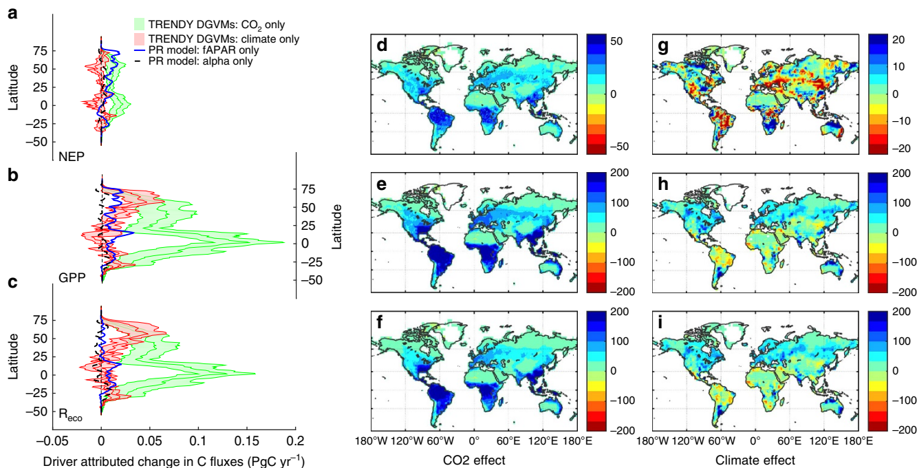
Figure 5 | Global distribution of change. (a–c) The latitudinal distribution of the effect of changes in different forcing factors on (a) net ecosystem production (NEP), (b) gross primary production (GPP) and (c) ecosystem respiration ( R_{eco} ). Shaded areas represent the mean and s.d. from the TRENDY ensemble of dynamic global vegetation models (DGVM) simulations with varying only \text{CO}_2 (green) or climate (red). Dashed lines in a–c show the effect of changes in vegetation (or the fraction of absorbed radiation (fAPAR), blue) and water availability (Alpha, black) estimated using a diagnostic coupled photosynthesis-respiration (PR) model. (d–i) The spatial distribution of the influence of increasing atmospheric \text{CO}_2 and changes in global climate on total rates of NEP (d,g), GPP (e,h) and total ecosystem respiration (f,i) in \text{gC m}^{-2} per year. Effects are estimated based on the difference between the 15-year periods of 1901–1915 and 1995–2010.
