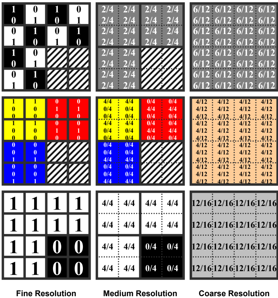
Figure 2 Example data where the fine resolution maps have four rows and four columns of pixels. The top row of maps shows the reference data which have two categories. The middle row of maps shows the comparison data which have three categories. The bottom row of maps shows the pixel weights which mask the lower right quadrant. The three columns show three grain sizes of fine, medium, and coarse.
