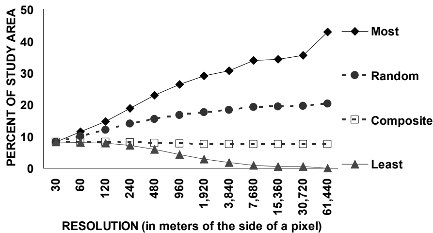
Figure 7 Association of the Forest category in 1971 map to the Built category in the 1999 map at multiple resolutions for the PIE data.
