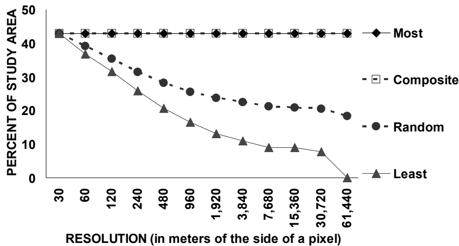
Figure 8 Association of the Built category in 1999 map to the Built category in the 1999 map at multiple resolutions for the PIE data.
